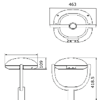
GARDEN LIGHT
