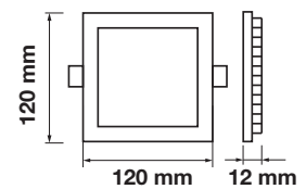
Cutting Size: 110x110mm
