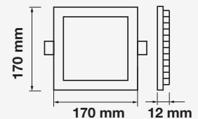
Cutting Size: 160x160mm
