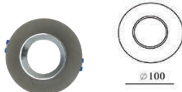
Fitting-Recessed-1XGU10
